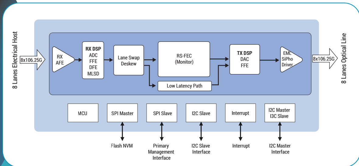
Figure1: O-Wave AW100-T Functional Block Diagram
